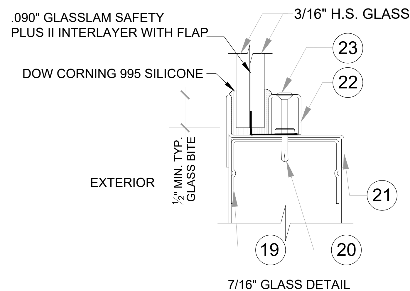
7/16" GLASS DETAIL
