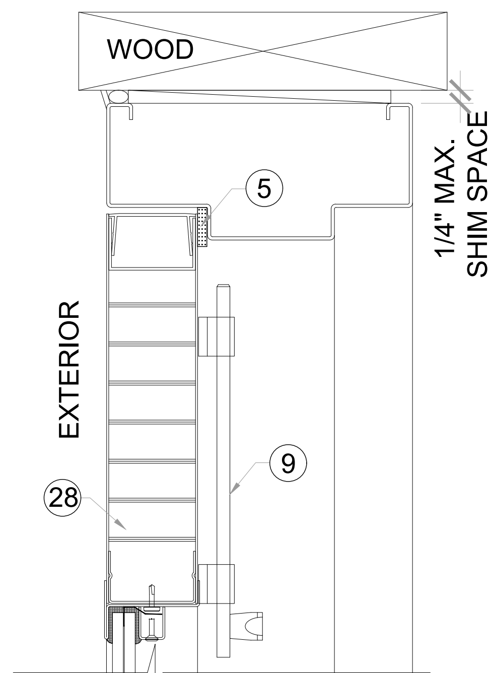
HEAD OPTION 3 A
