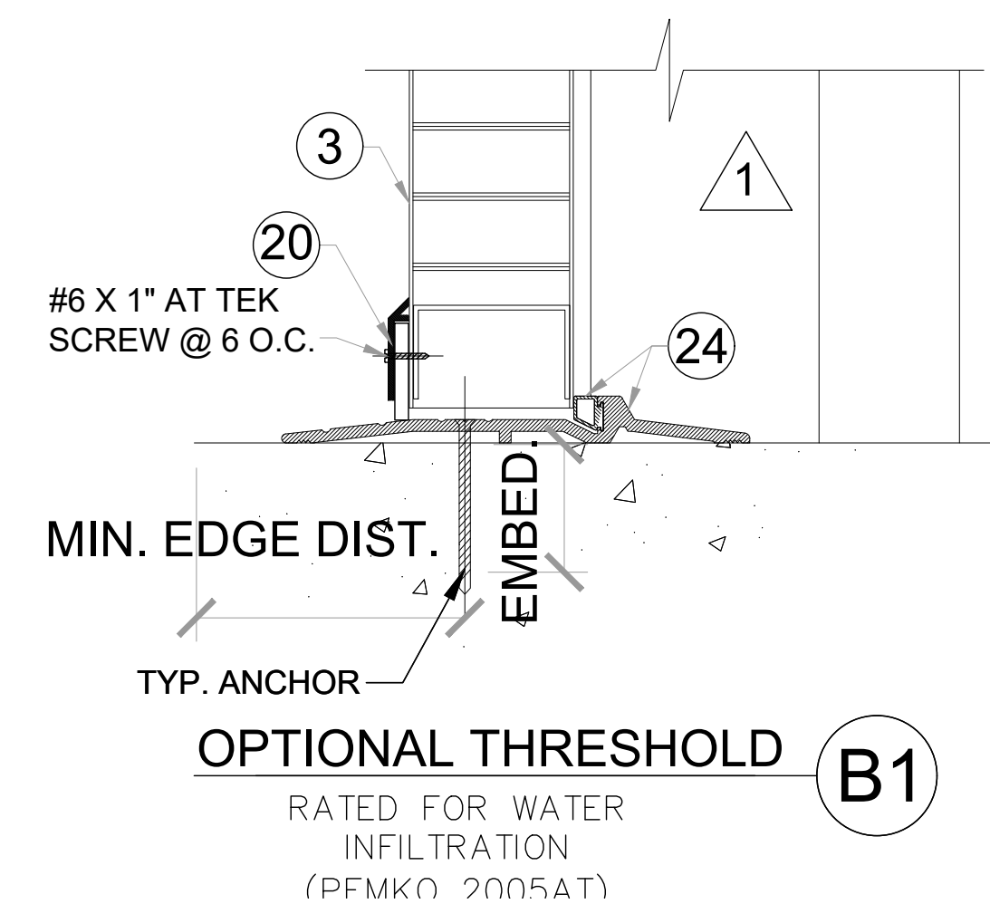
TYPICAL THRESHOLD B RATED FOR WATER INFILTRATION (PEMKO 177AT96)
