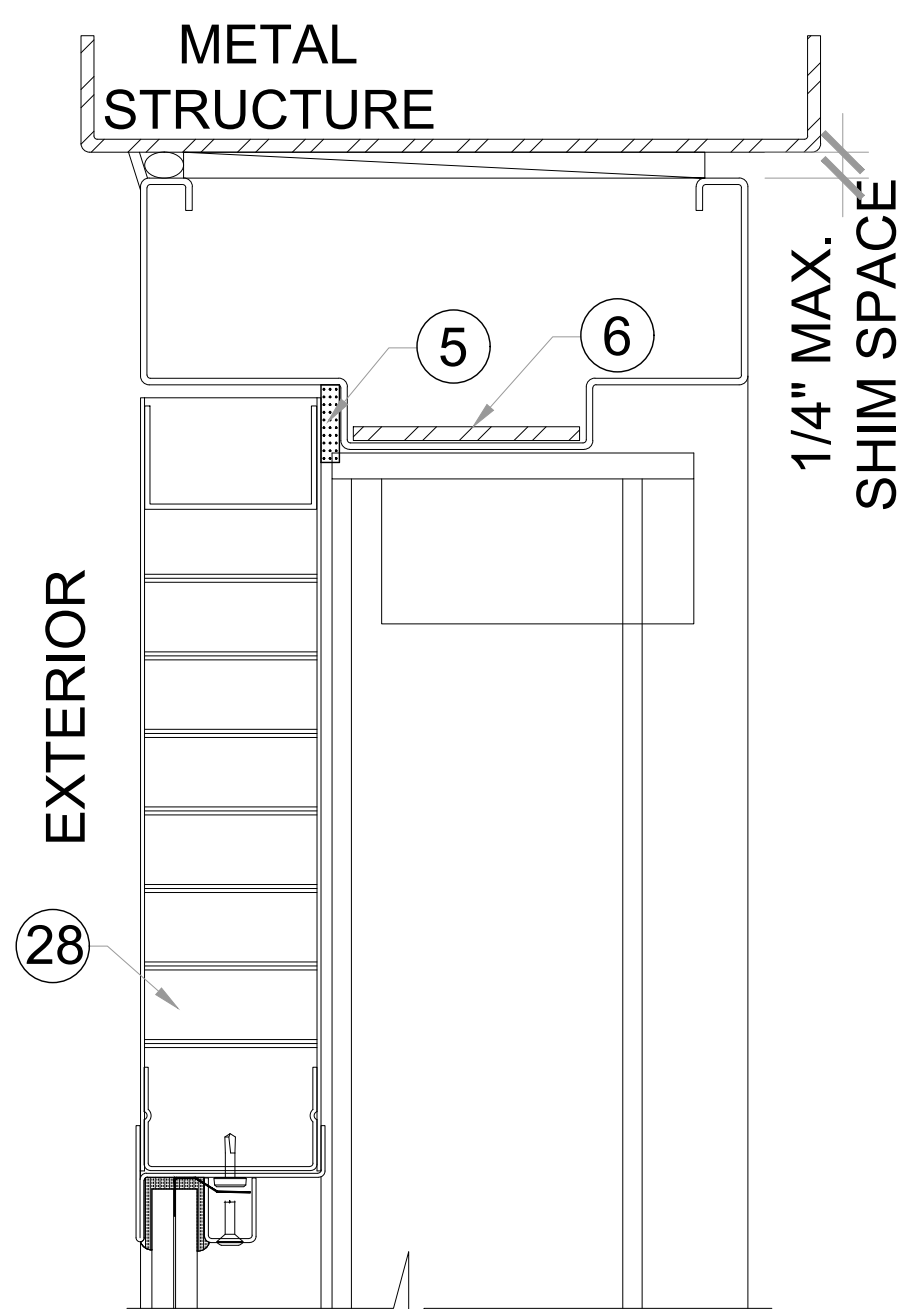
HEAD OPTION 2 A
