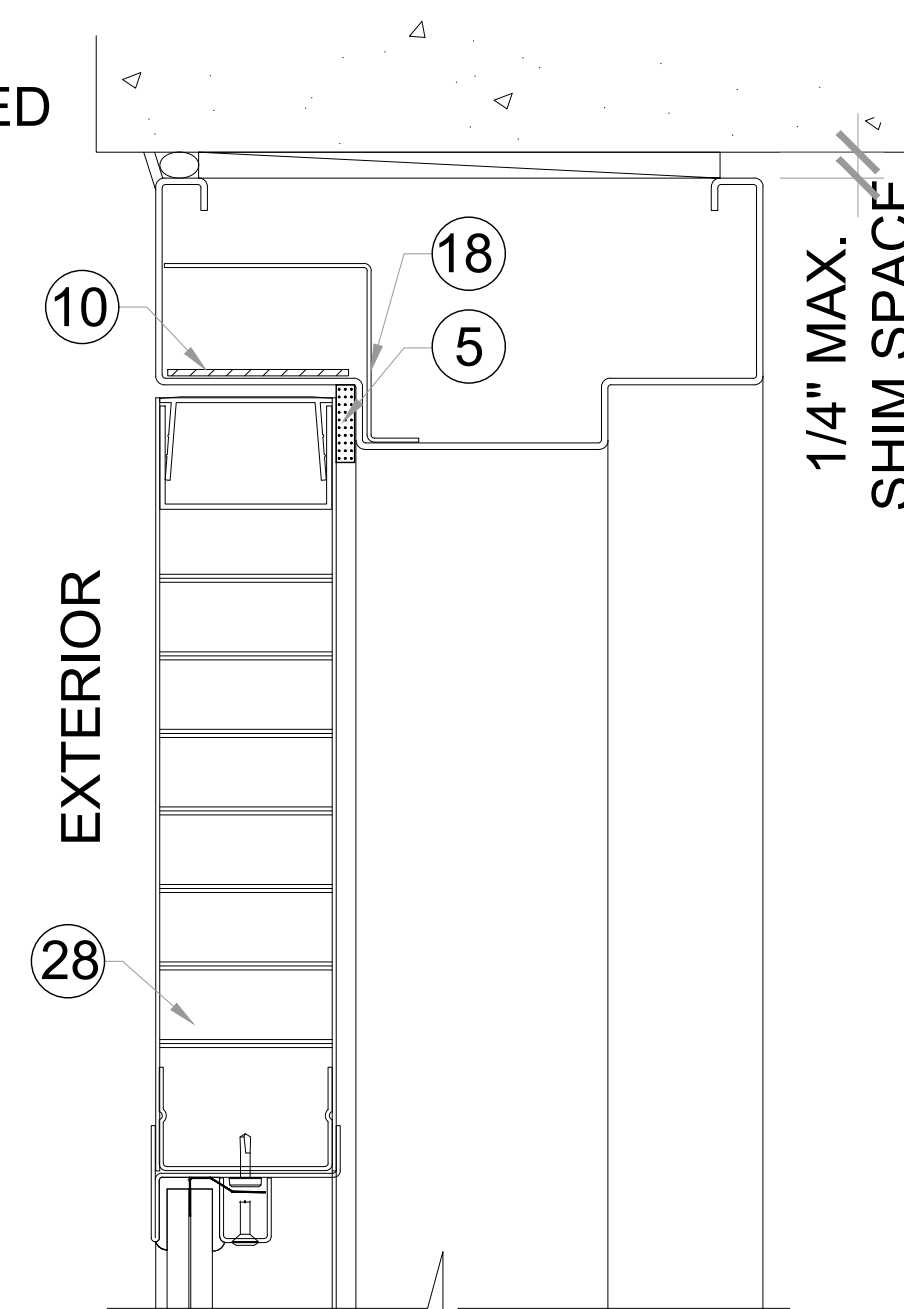
HEAD OPTION 5 A
