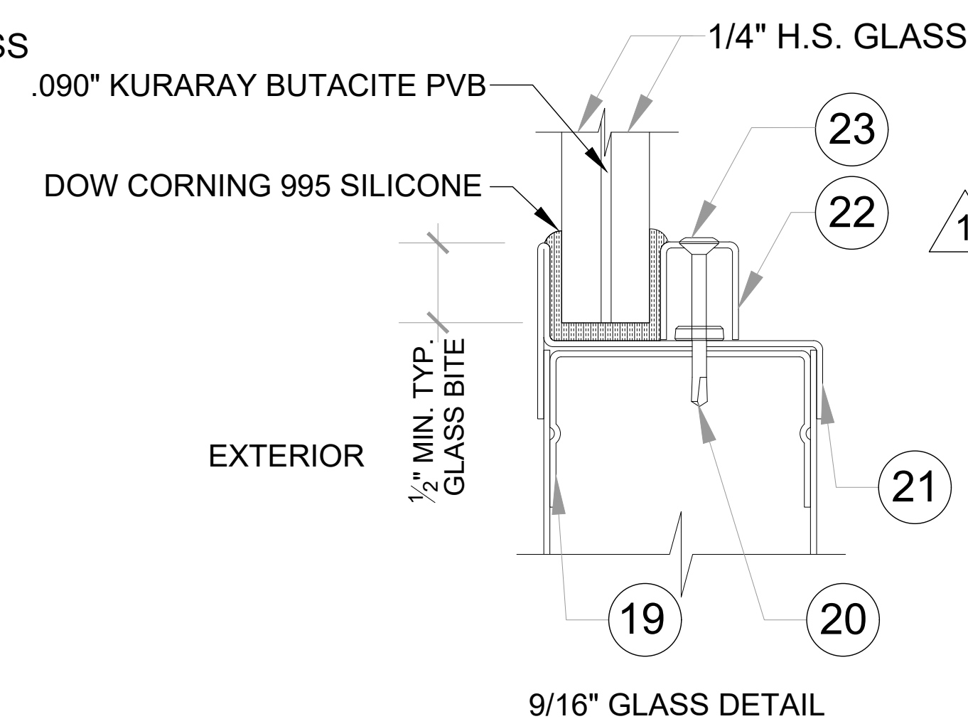
9/16" GLASS DETAIL
