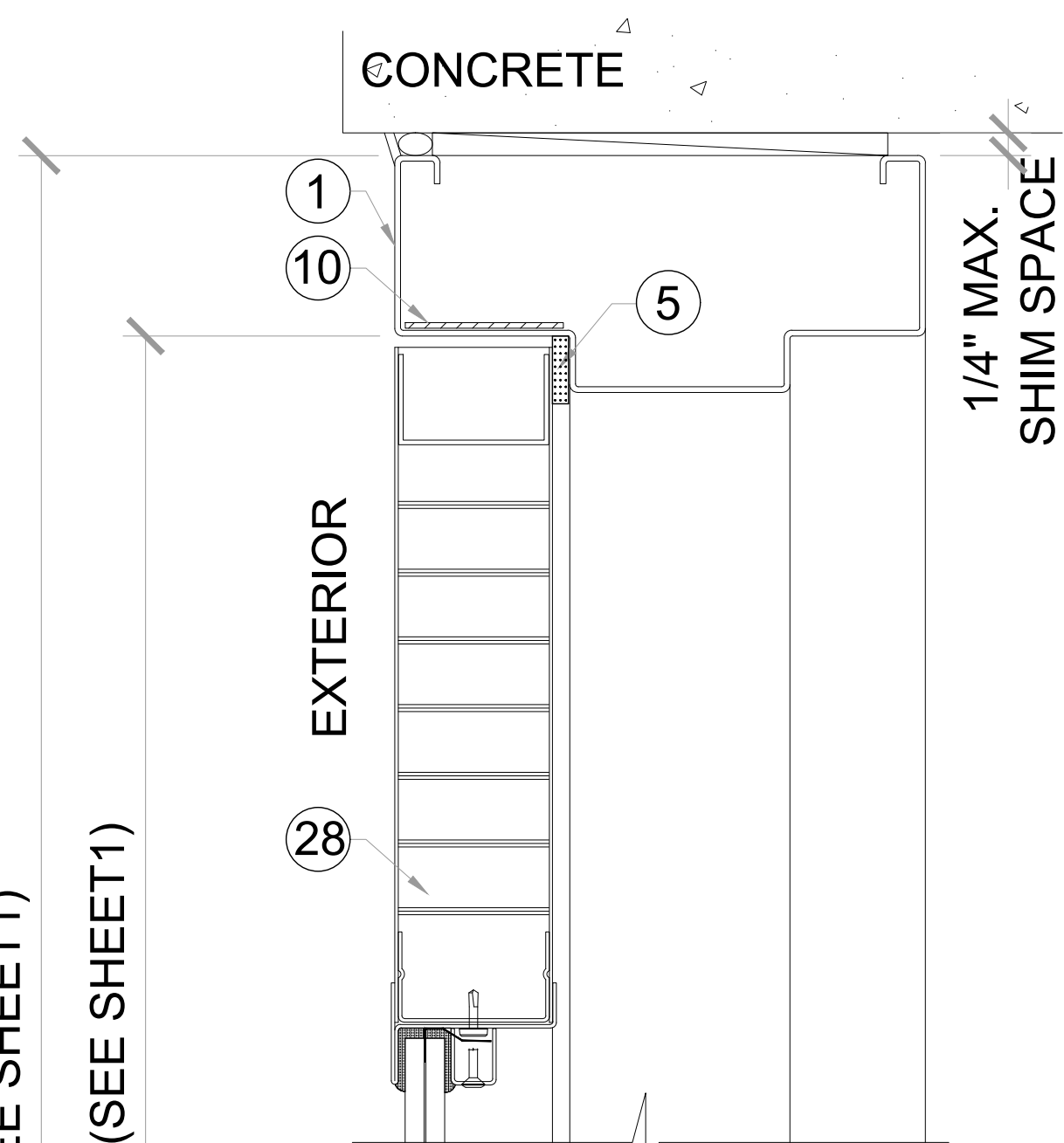
HEAD OPTION 1 A
