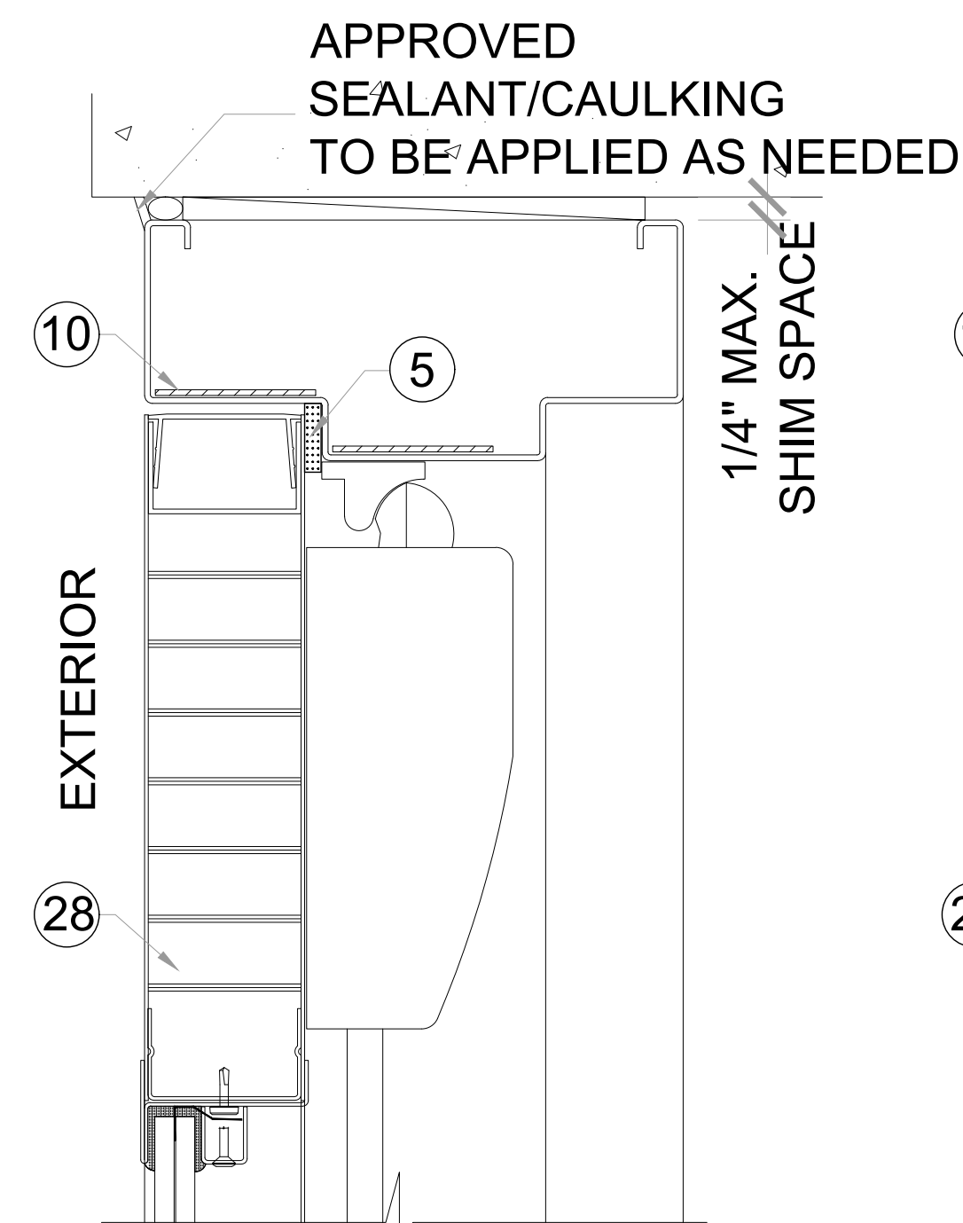
HEAD OPTION 4 A
