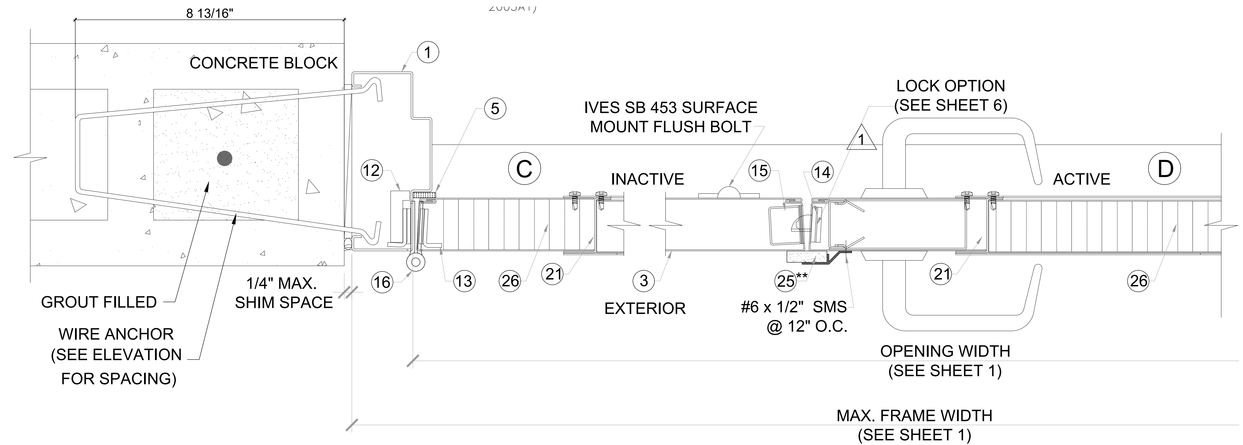
LOCK OPTION # 1 SERIES 8200 SARGENT MORTISE LOCK W/ SURFACE BOLTS (INACTIVE)
